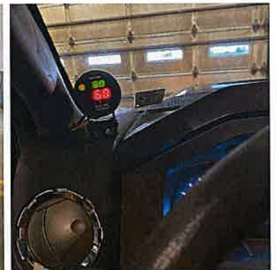
Left: Plow with adaptive blade retrofit to help remove ice from the road, using less salt. Right: Road temperature sensor to better gauge when to apply salt reducing the amount applied.
